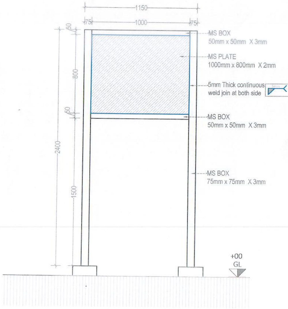
SIGN BOARD DETAIL DESIGN
